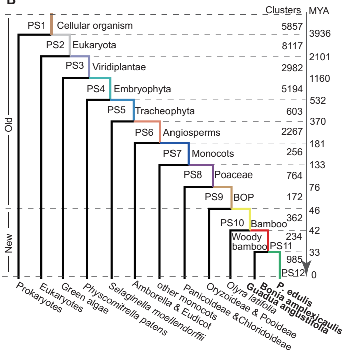
FIG. 1. Morphological character and phylostratigraphic age of Phyllostachys edulis . (A) Comparison of the growth pattern of grass and woody bamboo. (B) Phylostratigraphic ages distribution of P. edulis . Numbers denote the number of nonredundant gene clusters per phylostratum (PS1–PS12). The tree stratifies species by major evolutionary innovations, from the emergence of simple unicellular organisms up to P. edulis . The dating of phylogenetic tree is from TimeTree (Kumar et al. 2017). (C) Number of genes per phylostratum. (D) Gene fixation rate per PS. (E) Gene copies distribution of each cluster.
